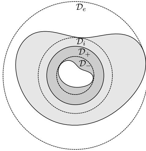
Fig. 2 – The four concentric disks introduced in Hypothesis 3.1. We recall also the definition of the annuli \mathcal{C}_e = \mathcal{D}_e \setminus \overline{\mathcal{D}_+} and \mathcal{C}_+ = \mathcal{D}_+ \setminus \overline{\mathcal{D}_-} .
