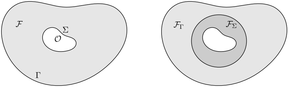
Fig. 1 – On the left: The domains and the boundaries; \mathcal{G} = \mathcal{F} \cup \overline{\mathcal{O}} . On the right: the partition of \mathcal{F} into \mathcal{F}_\Sigma (a neighborhood of the boundary \Sigma ) and \mathcal{F}_\Gamma .
