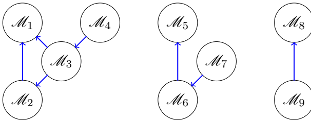
Fig. 2 – Representation of a graph \mathcal{G} with 9 vertices. The sinks of the graph are \mathcal{M}_1 , \mathcal{M}_5 , and \mathcal{M}_8 . A Barabanov norm exists, according to Theorem 14, if and only if \mathcal{M} is nondefective and
