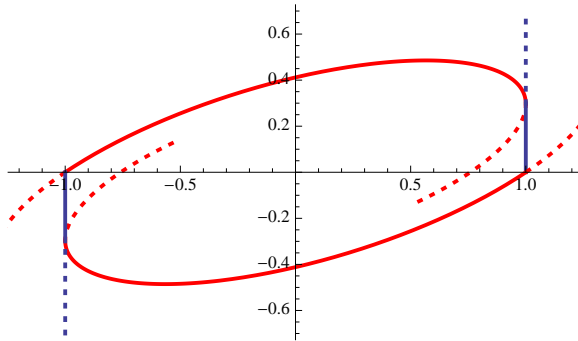
Fig. 1 – Barabanov norm construction for the switched system of Example 12.
