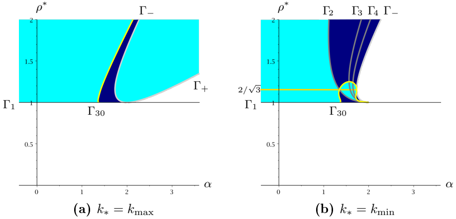
Fig. 3 – Bifurcations of steady periodic solutions in the case of anomalous dispersion. In the (\alpha, \rho^*) -plane, the bifurcation is supercritical ( c_{30} < 0 ) in the lighter shaded regions (light blue online) and subcritical ( c_{30} > 0 ) in the darker shaded regions (navy blue online). In the case k_* = k_{\min} , we also represent the curves \Gamma_n , for n = 2, 3, 4 , along which resonances occur, and the line \rho^* = 2/\sqrt{3} along which c_{11} changes sign.
