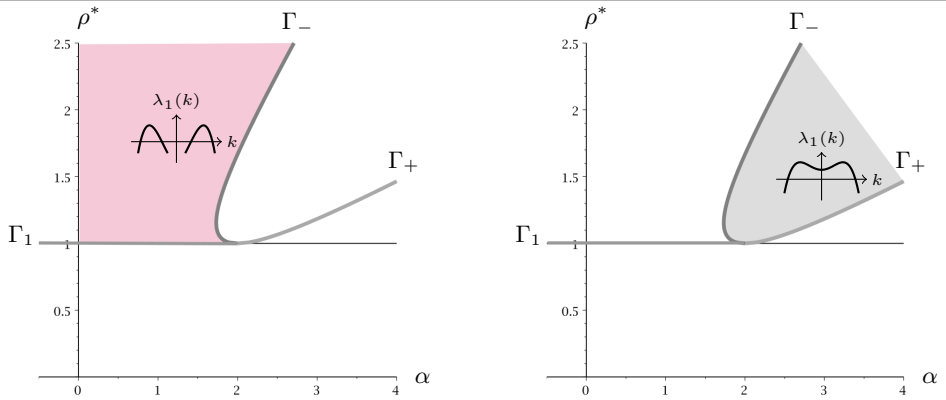
Fig. 2 – Stability of constant solutions in the case of anomalous dispersion. In the (\alpha, \rho^*) -plane, the shaded regions represent the values for which a constant solution with \rho^* = |\psi^*|^2 is Turing unstable (left plot) and zero-mode unstable (right plot). The insets show a typical shape of the largest eigenvalue \lambda_1(k) in these instability regions.
