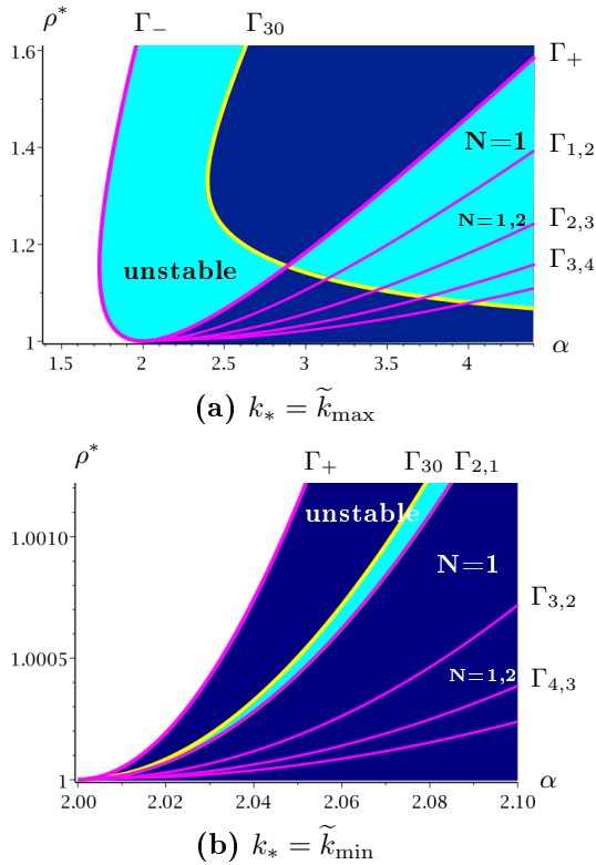
Fig. 6 – Stability of steady periodic solutions in the case of normal dispersion. In the (\alpha, \rho^*) -plane, the steady periodic solutions are background stable for subharmonic perturbations with periods 2\pi N/k_* for the values of N as indicated, and unstable otherwise. In the lighter shaded regions (light blue online) they are shape stable, whereas in the darker shaded regions (navy blue online) they are shape unstable. The curves \Gamma_{n,N} are defined by (4.4) in the case k_* = \tilde{k}_{\max} and by (4.3) in the case k_* = \tilde{k}_{\min} .
