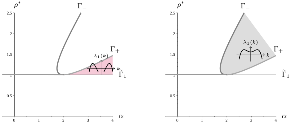
Fig. 5 – Stability of constant solutions in the case of normal dispersion. In the (\alpha, \rho^*) -plane, the shaded regions represent the values for which a constant solution with \rho^* = |\psi^*|^2 is Turing unstable (left plot) and zero-mode unstable (right plot). The insets show a typical shape of the largest eigenvalue \lambda_1(k) in these instability regions.
