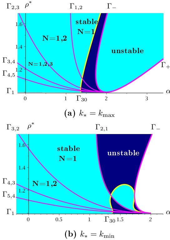
Fig. 4 – Stability of steady periodic solutions in the case of anomalous dispersion. In the (\alpha, \rho^*) -plane, the steady periodic solutions are background stable for subharmonic perturbations with periods 2\pi N/k_* for the values of N as indicated, and unstable otherwise. In the lighter shaded regions (light blue online) they are shape stable, whereas in the darker shaded regions (navy blue online) they are shape unstable. The curves \Gamma_{n,N} are defined by (4.3) in the case k_* = k_{\max} and by (4.4) in the case k_* = k_{\min} .
