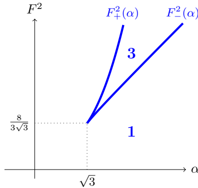
Fig. 1 - Number of constant solutions of the Lugiato-Lefever equation (1.1): three solutions in the region between the curves F^2 = F_{\pm}^2(\alpha) , two solutions along the curves, and one solution otherwise.
