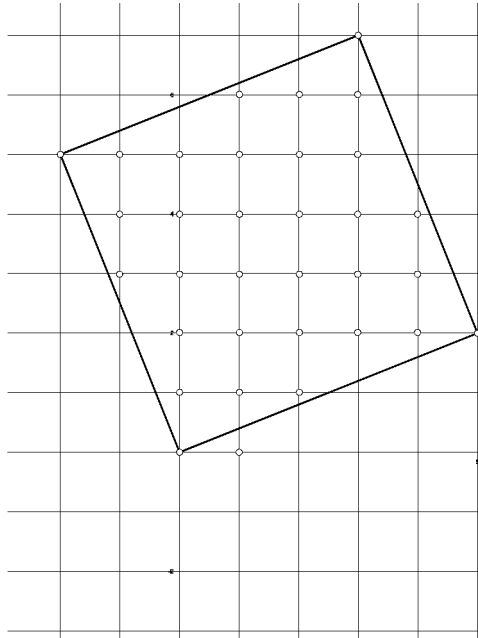
Fig. 1 – Square with a = 5 and b = 2 .
